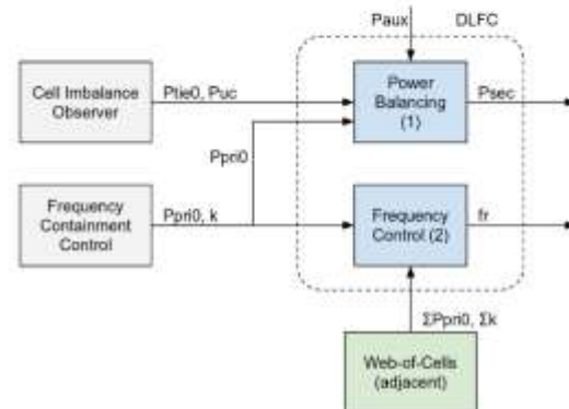
Fig. 1: Signal flow for the BRC/FCC parts of the DLFC.
