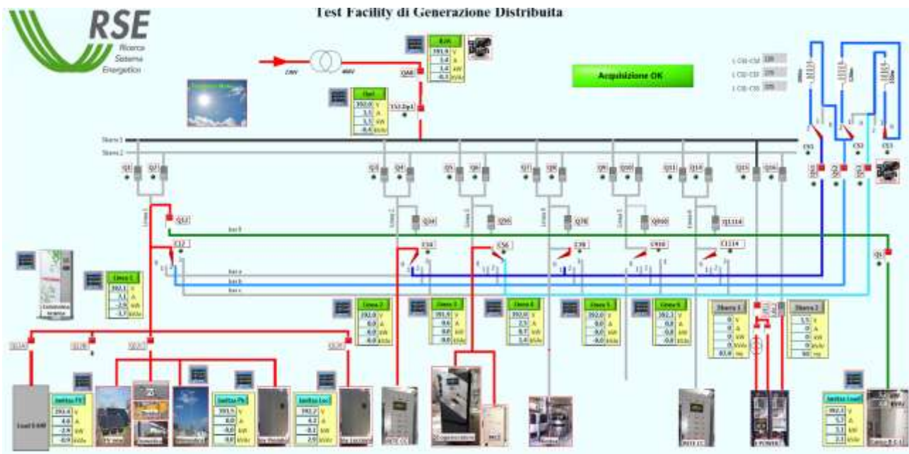
Figure 3.7: DER-TF microgrid of RSE
