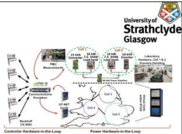
Fig. 5. C-HiL and P-HiL validation setup
