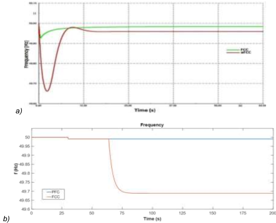
Figure 4.2: Examples of requirement of tuning for proposed fuzzy FCC –
