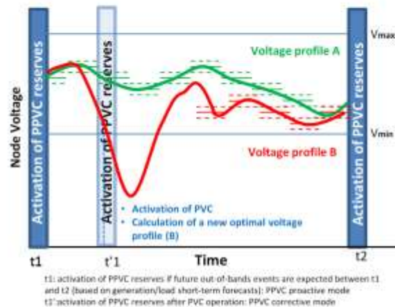
Fig. 1. Operation of the PVC/PPVC strategy (proactive/corrective)
