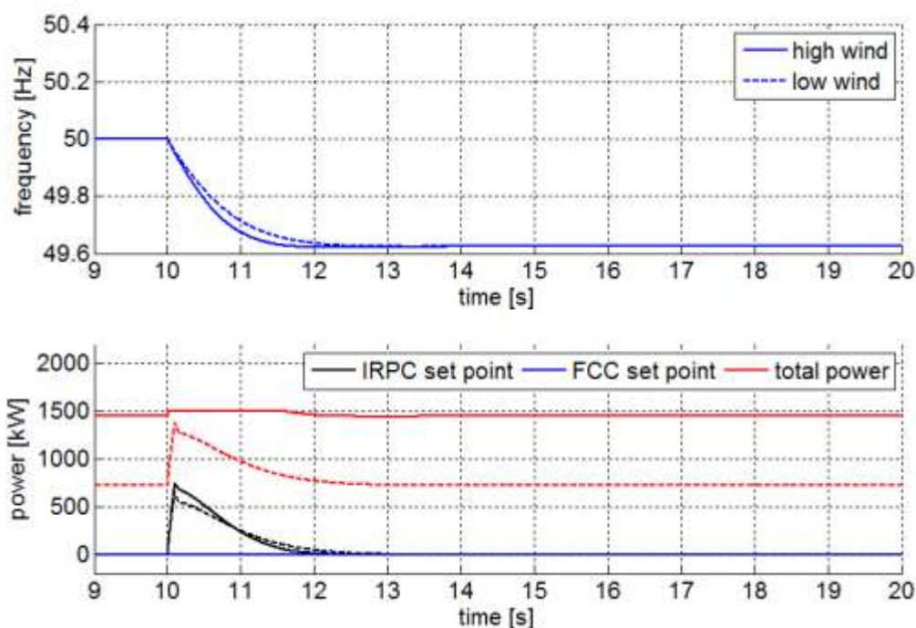
Figure 4.33: RPC and FCC contribution of the wind turbine after load increase, IEE
