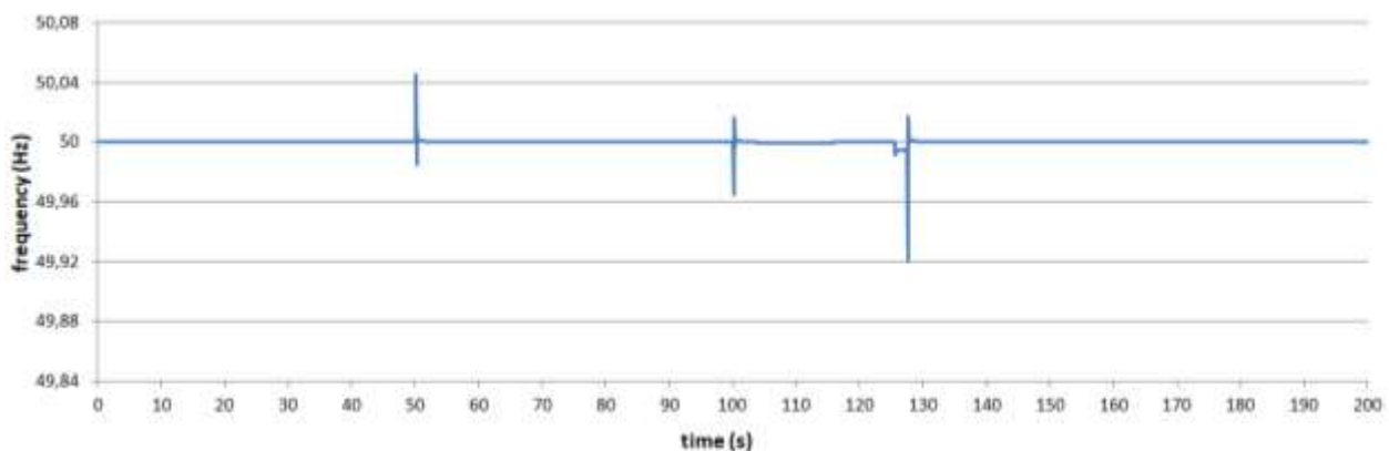
Figure 4.22: Simulation results showing the frequency response of the system in Test 4
