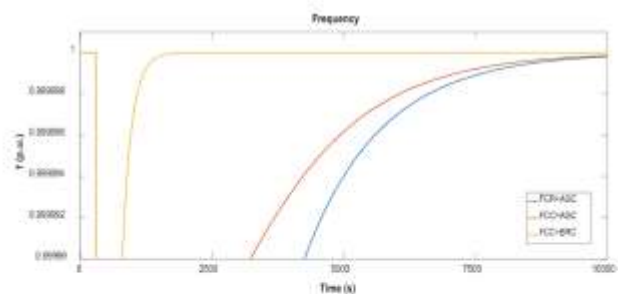
Fig. 3. Frequency of the system (10000s)
