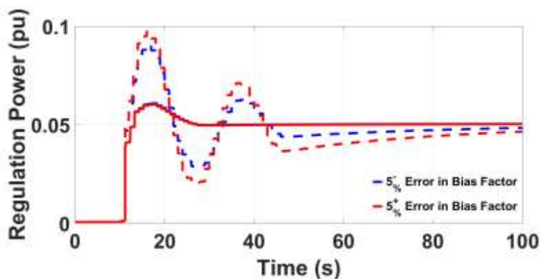
Figure 4.11: Usage of ACE within BCL
