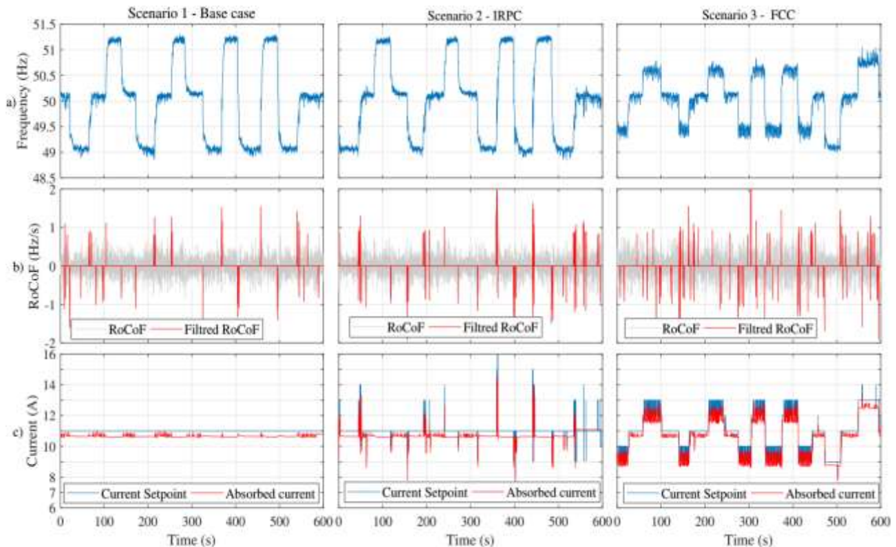
Figure 4.37: Study Case 1 (load steps) – (a) Frequency, (b) RoCoF, and (c) EV1's set-pint vs. absorbed current, DTU
