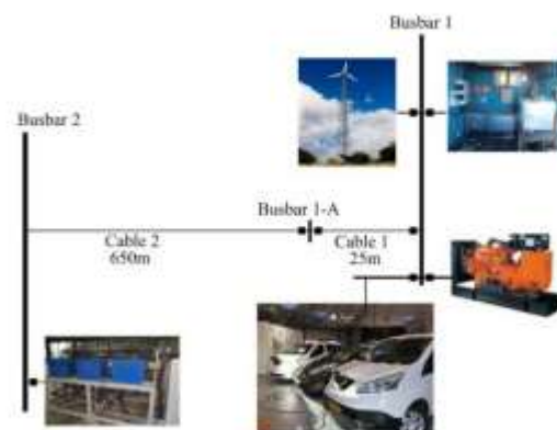
Fig. 2. Web of Cells representation
