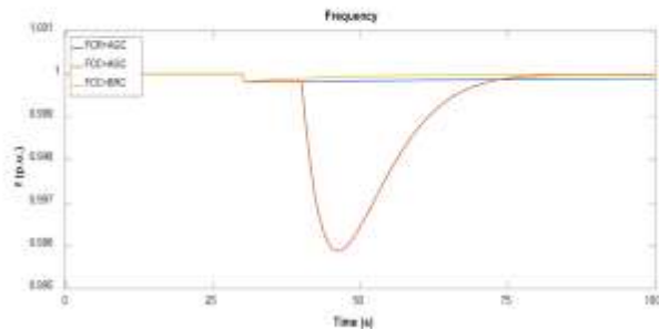
Fig. 2. Frequency of the system (100s)
