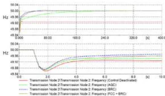
Fig. 4. FCC/BRC impact on frequency response.
